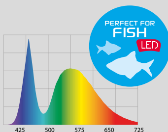
SUNNY LED source
