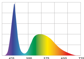
LEDDY SLIM MARINE 10000K
